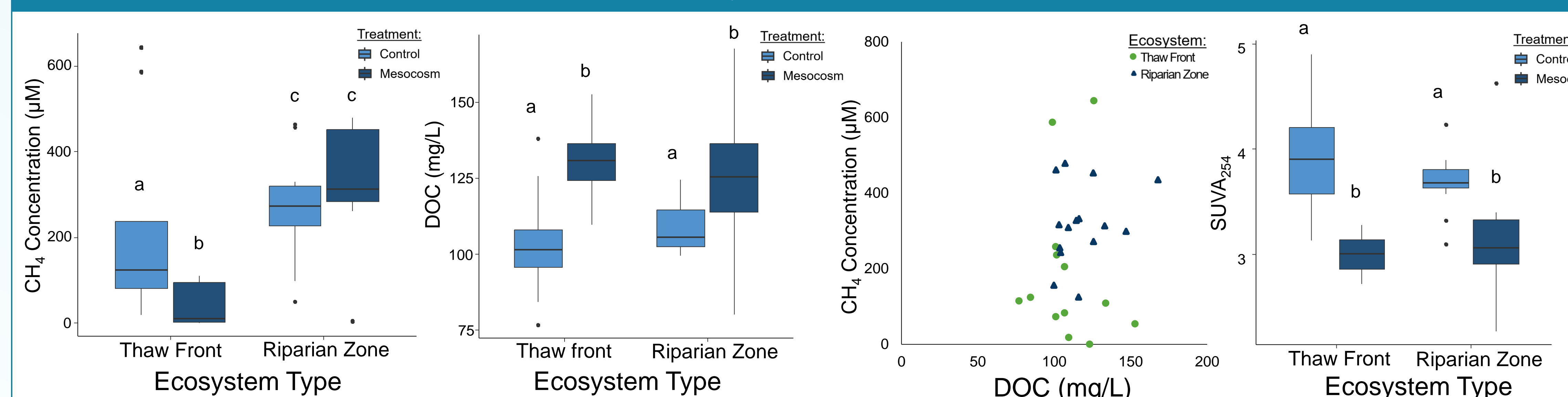
Figure 1: CH 4 concentrations at the thaw front and riparian zone for control plots and mesocosm sites. Control plots had higher concentrations at the thaw front (p<0.01), and no difference between plots in the riparian (p=0.09). Concentrations were higher in the riparian zone than the thaw front (p<0.001). Difference letters indicate significant differences (p < 0.05).
