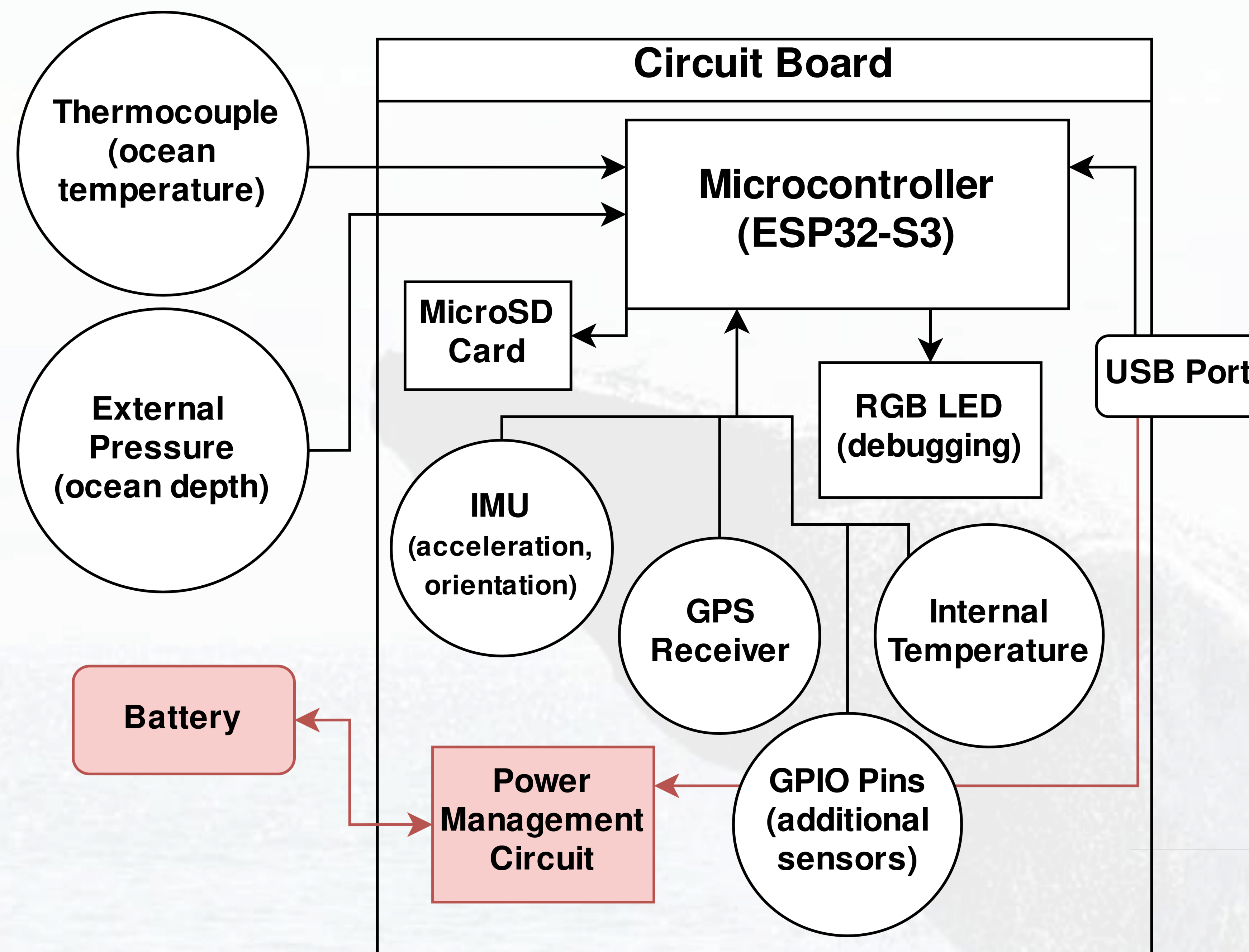
Figure 1. Sensor Payload Final Block Diagram
